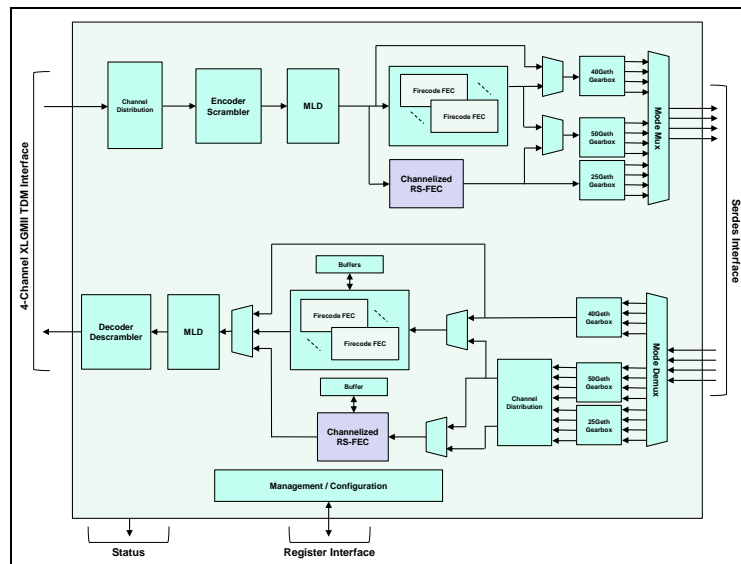
Core Block Diagram
